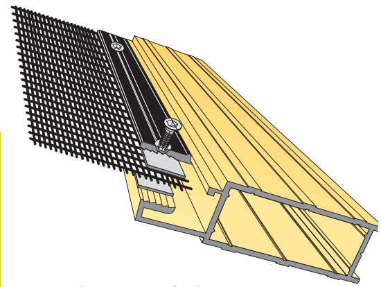
Only Crimsafe drives a screw right through mesh and frame – for unbeatable strength
